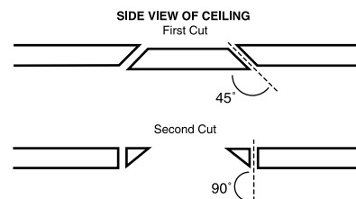
Diagram 1: Ceiling Cut Out
