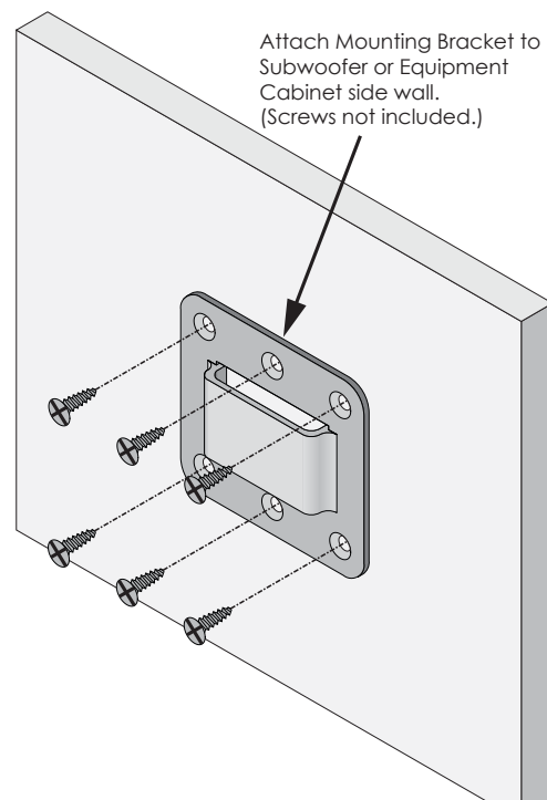
Figure 8 SA 2.1 Receiver Mounting Bracket
