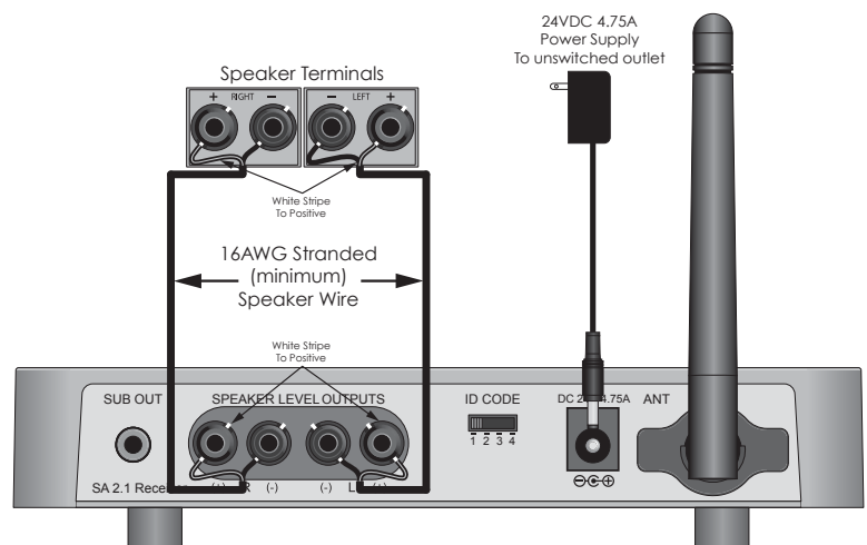
Figure 12 SA 2.1 Receiver Speaker Level Output Connections
