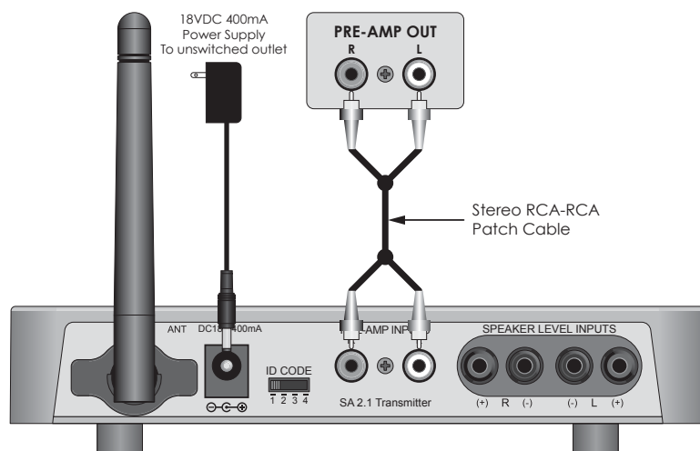
Figure 13 SA 2.1 Transmitter Pre-amp Input Connections
